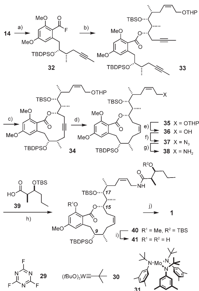
Scheme 4. a) 29 , pyridine, \text{CH}_2\text{Cl}_2 , -25^\circ\text{C} ; b) 25 , \text{NaN}(\text{SiMe}_3)_2 , THF, -78^\circ\text{C} \rightarrow \text{RT} ; 91% (over both steps); c) 31 (10 mol%), toluene, \text{CH}_2\text{Cl}_2 , 80^\circ\text{C} , 87%; d) Lindlar catalyst, \text{H}_2 (1 atm), EtOAc, quinoline, 96%; e) \text{MgBr}_2 \cdot \text{Et}_2\text{O} , \text{Et}_2\text{O} , 93%; f) [\text{Zn}(\text{N}_3)_2 \cdot (\text{pyridine})_2] , \text{PPh}_3 , DIAD, toluene, 0^\circ\text{C} , 65%; g) \text{PPh}_3 , aq THF, 50^\circ\text{C} , 91%; h) 39 , HBTU, HOAt, (i\text{Pr})_2\text{NEt} , DMF, 64%; i) \text{BCl}_3 , \text{CH}_2\text{Cl}_2 , -78^\circ\text{C} , 83%; j) aq HF (48% w/w), MeCN, 0^\circ\text{C} \rightarrow \text{RT} , 84%. HBTU = O -(benzotriazol-1-yl)- N,N,N',N' -tetramethyluronium hexafluorophosphate; HOAt = 1-hydroxy-7-azabenzotriazole.
